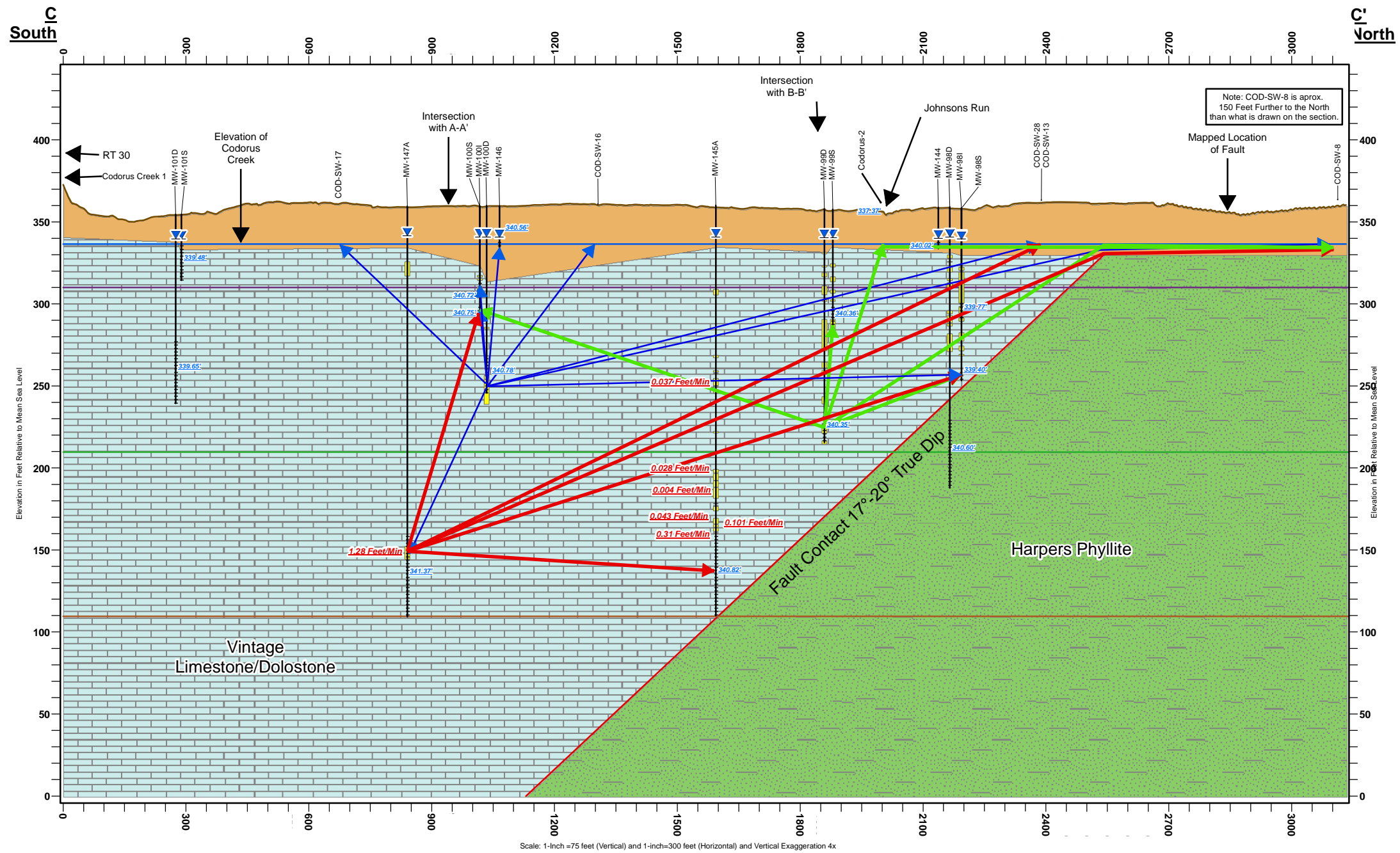
Scale: 1-Inch = 75 feet (Vertical) and 1-Inch = 300 feet (Horizontal) and Vertical Exaggeration 4x
